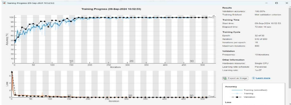
Figure 4: Training and testing phase for AlexNet
