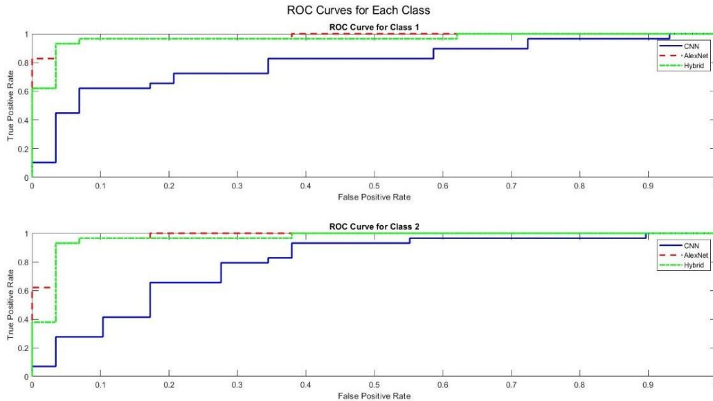
Figure 6: ROC curve
