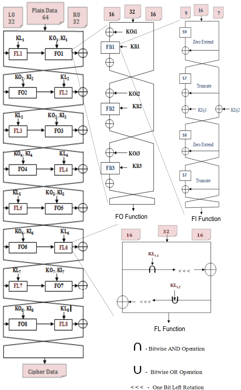
Figure 3: Architecture of KASUMI
